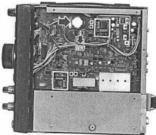
Fig. 6 Backup Switch
