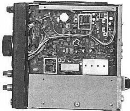
Fig. 4: TCXO-4 Installation
