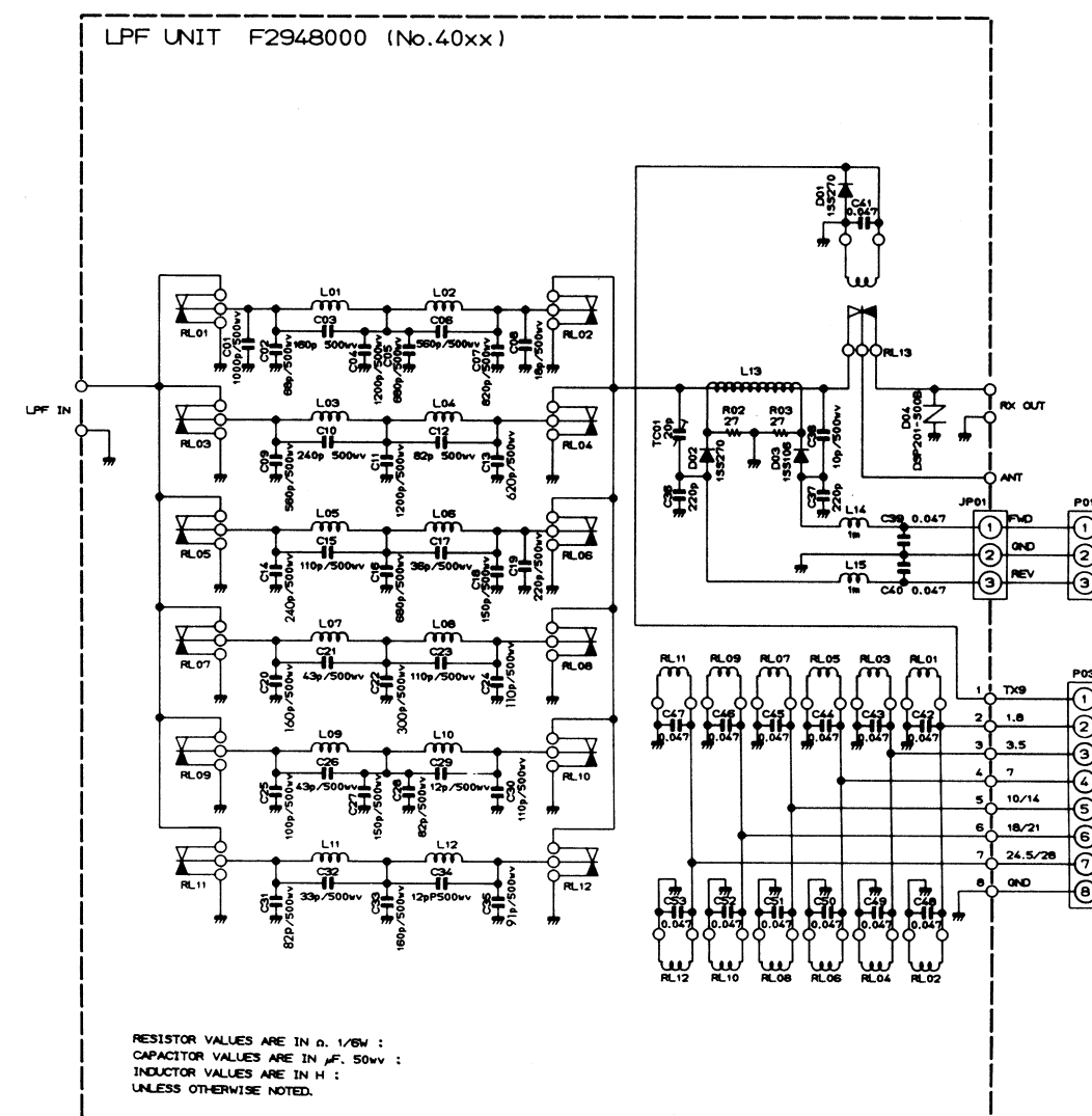
CIRCUIT DIAGRAM
