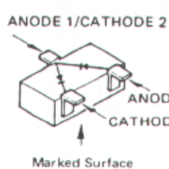
1SS226 (C3) (D201,209,211)
