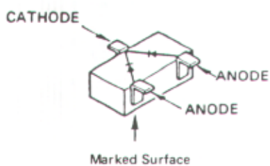
1SS184 (B3) (D208) SLM-23VMWS (D213)
