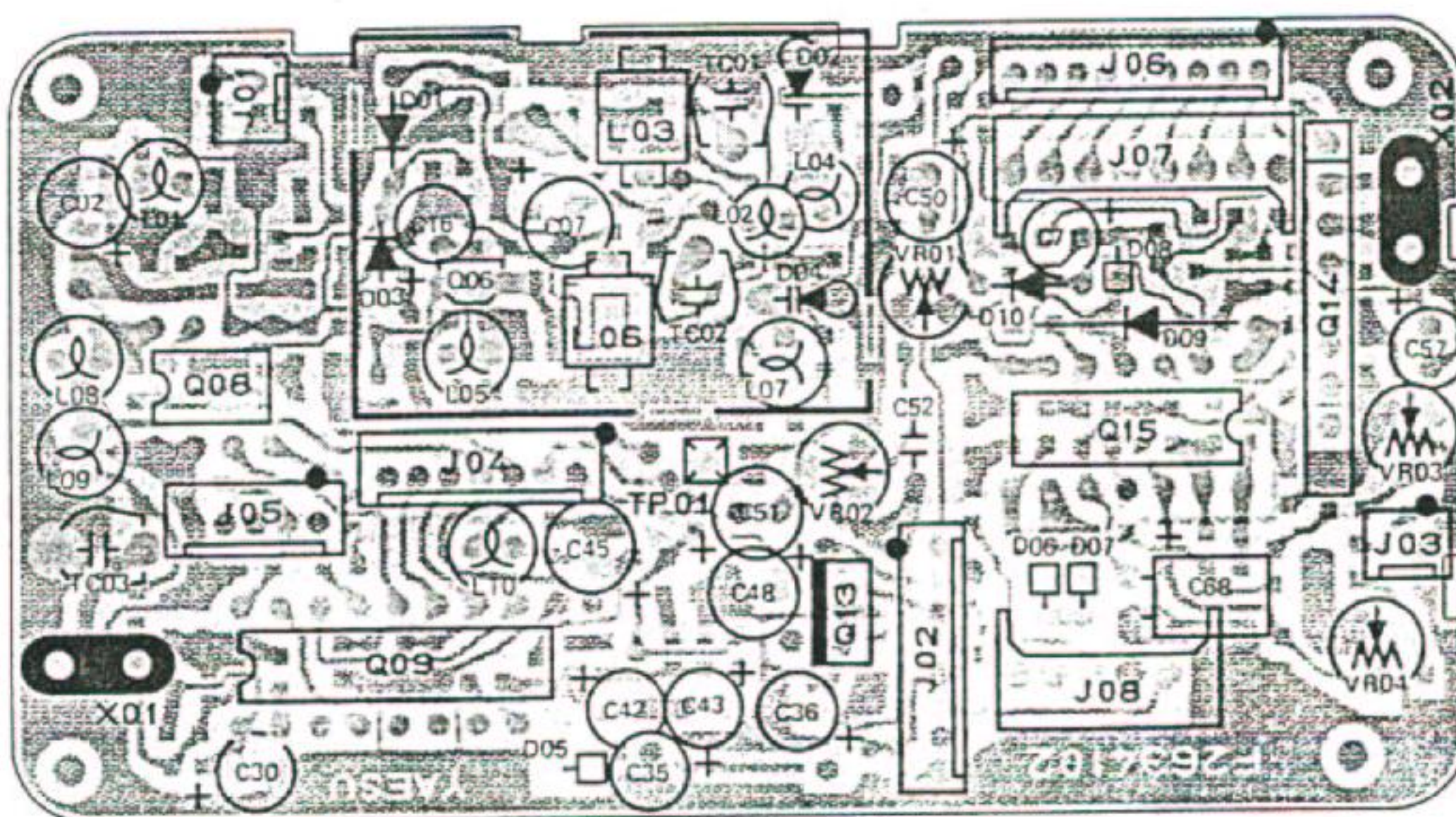
PLL UNIT (reverse view of "mixed component" side)
