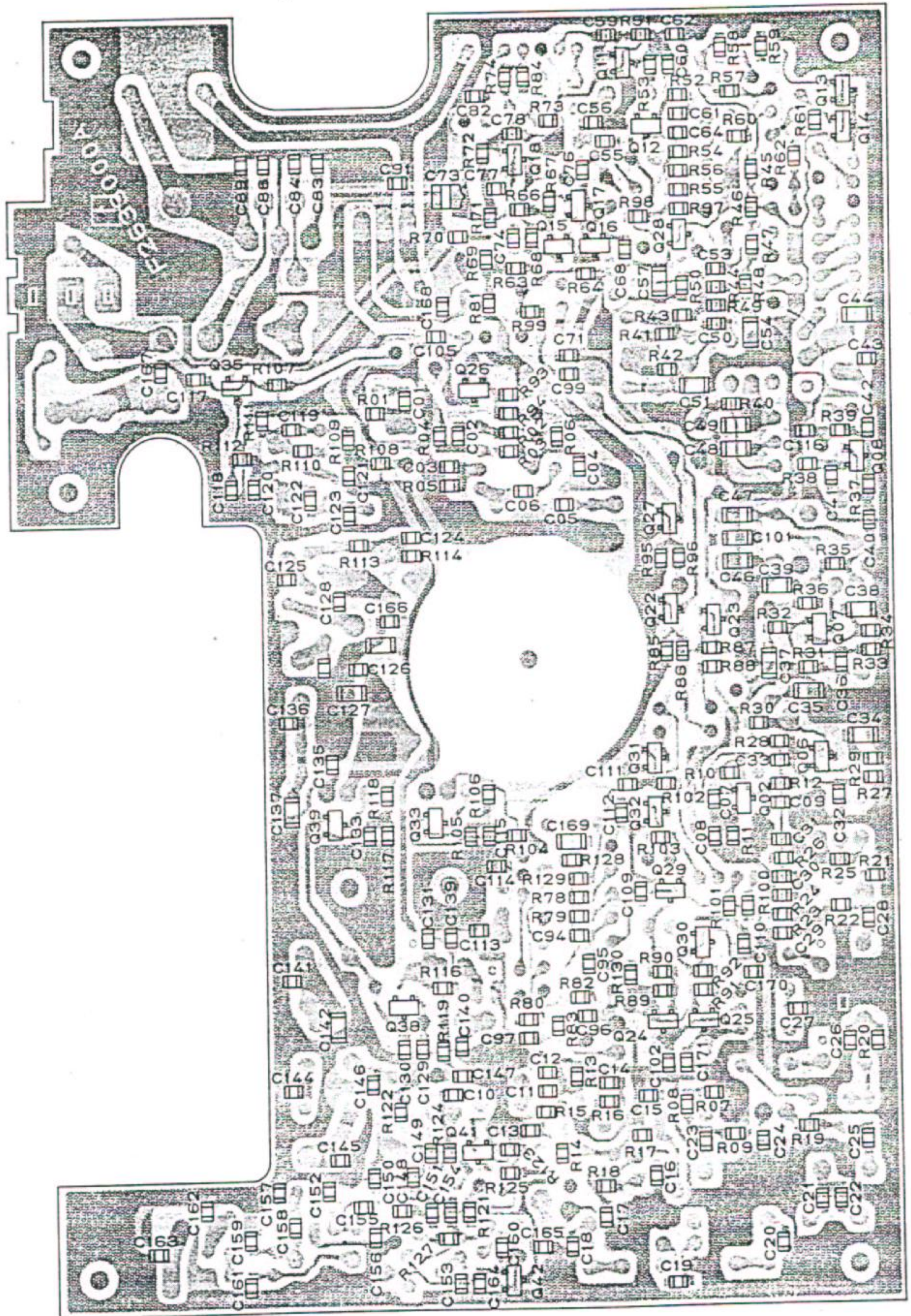
VHF UNIT (obverse view of "chip-only" side)
