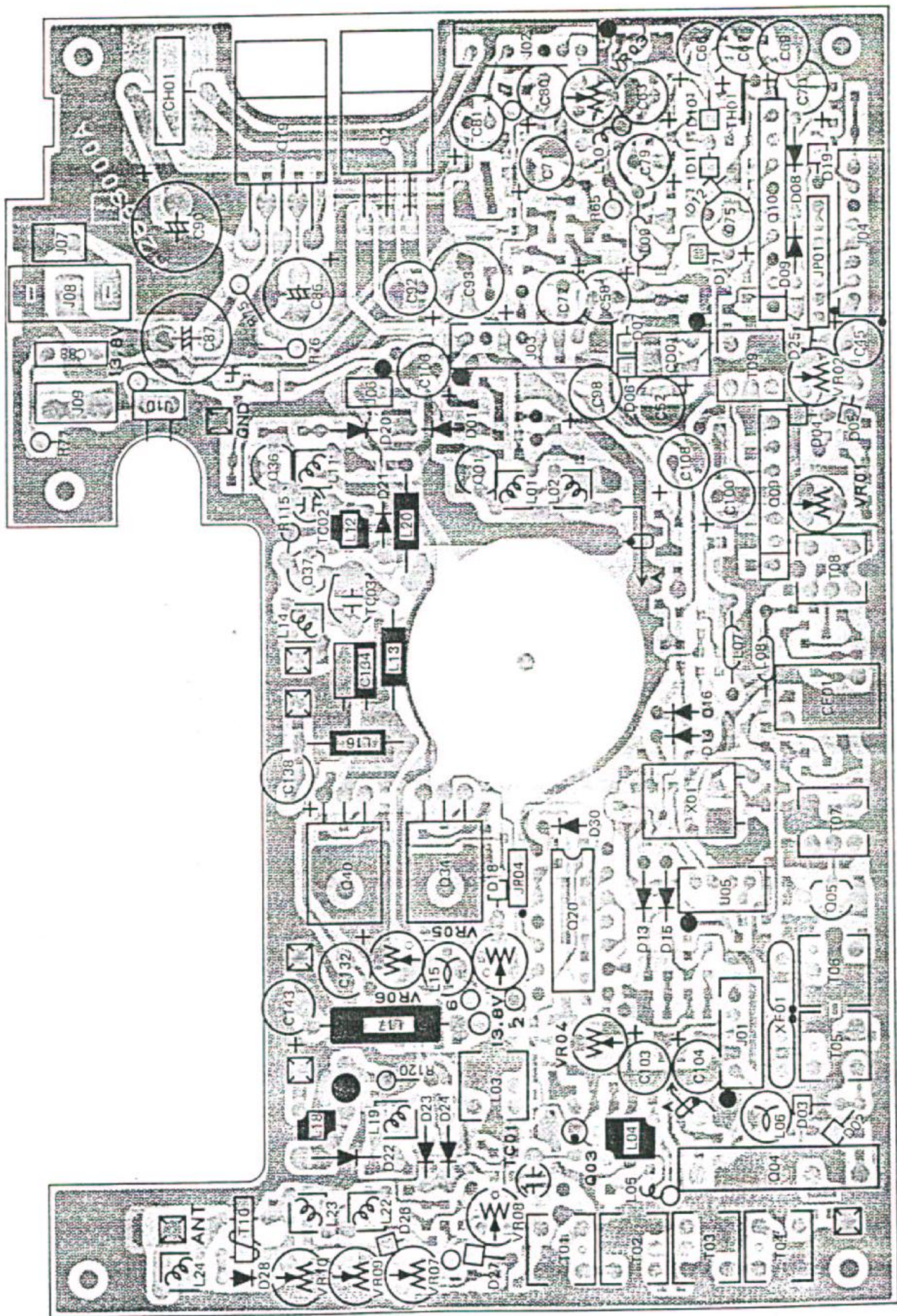
VHF UNIT (reverse view of "mixed component" side)
