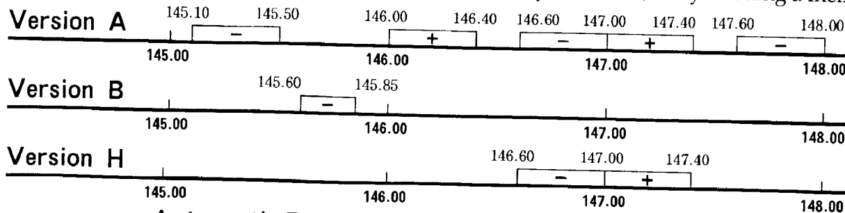
Automatic Repeater Shift - Repeater Subbands
