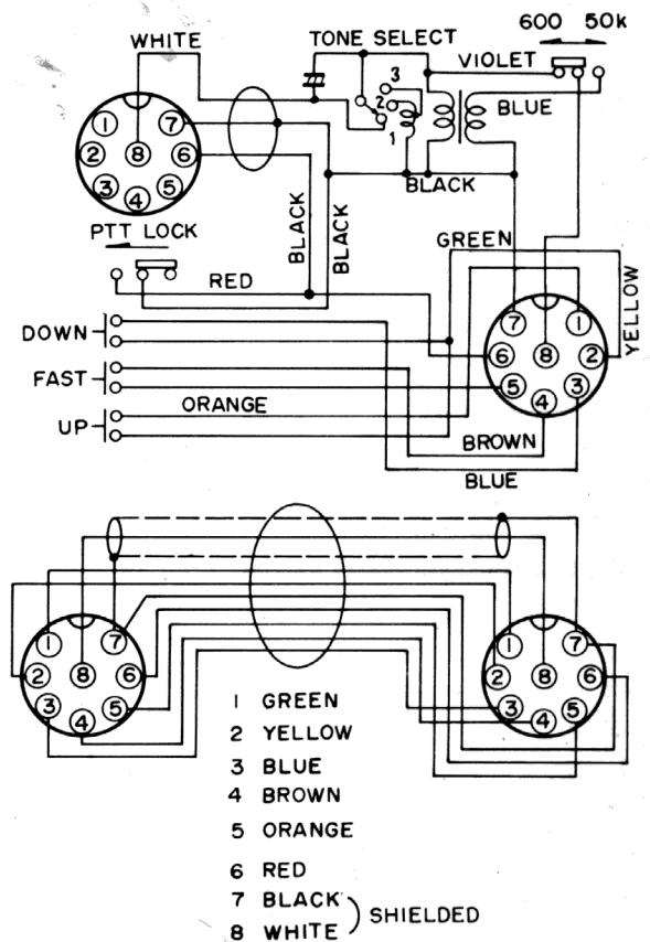
MD-1B8 MICROPHONE CONNECTIONS
