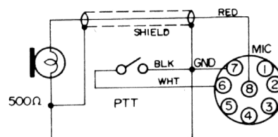
YM-37 MICROPHONE CONNECTIONS
