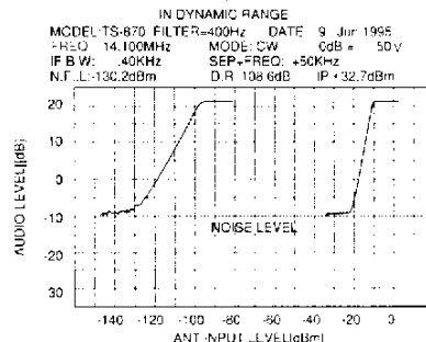
Figure 22: Dynamic range
