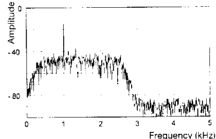
Figure 12: Audio spectrum for reception of 14.2MHz 120dBm signal in SSB mode (line enhancer off)
