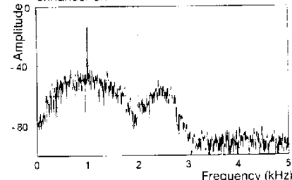
Figure 13: Audio spectrum with line enhancer on
