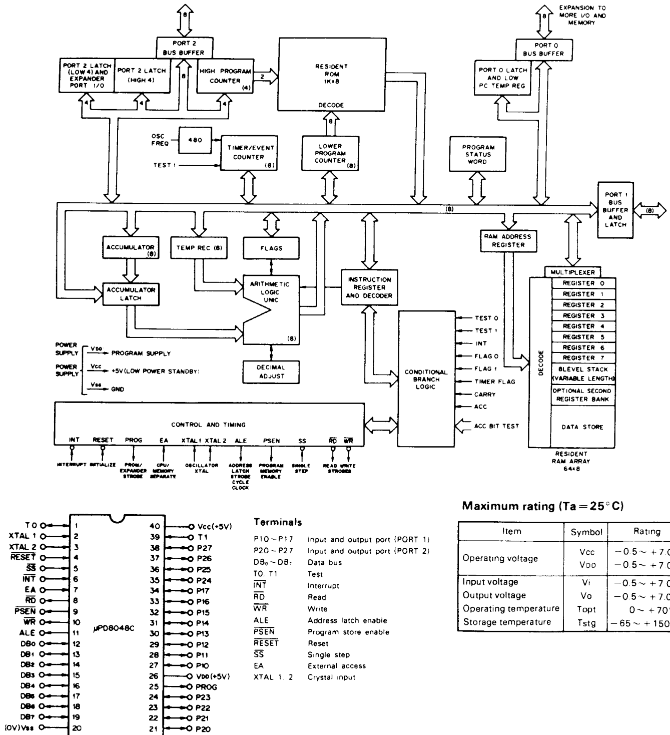
Fig. 13 \mu PD8048C-155 (DIGITAL UNIT, IC11)
