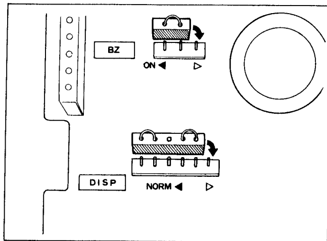
Fig. 3 Select Switches inside Case
