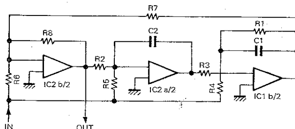
Fig. 2 Theoretical circuit diagram
