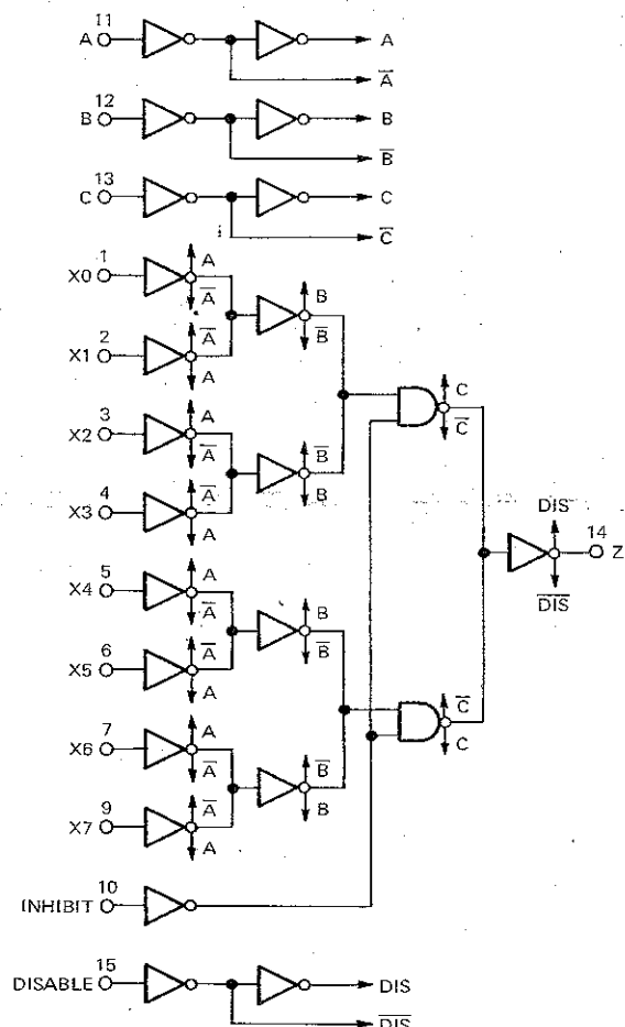
TC4512BP Block diagram (Control unit IC4,5)
