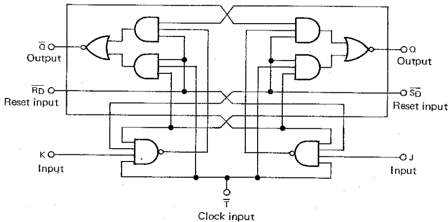
M74LS112AP Logic circuit (PLL unit IC5)
