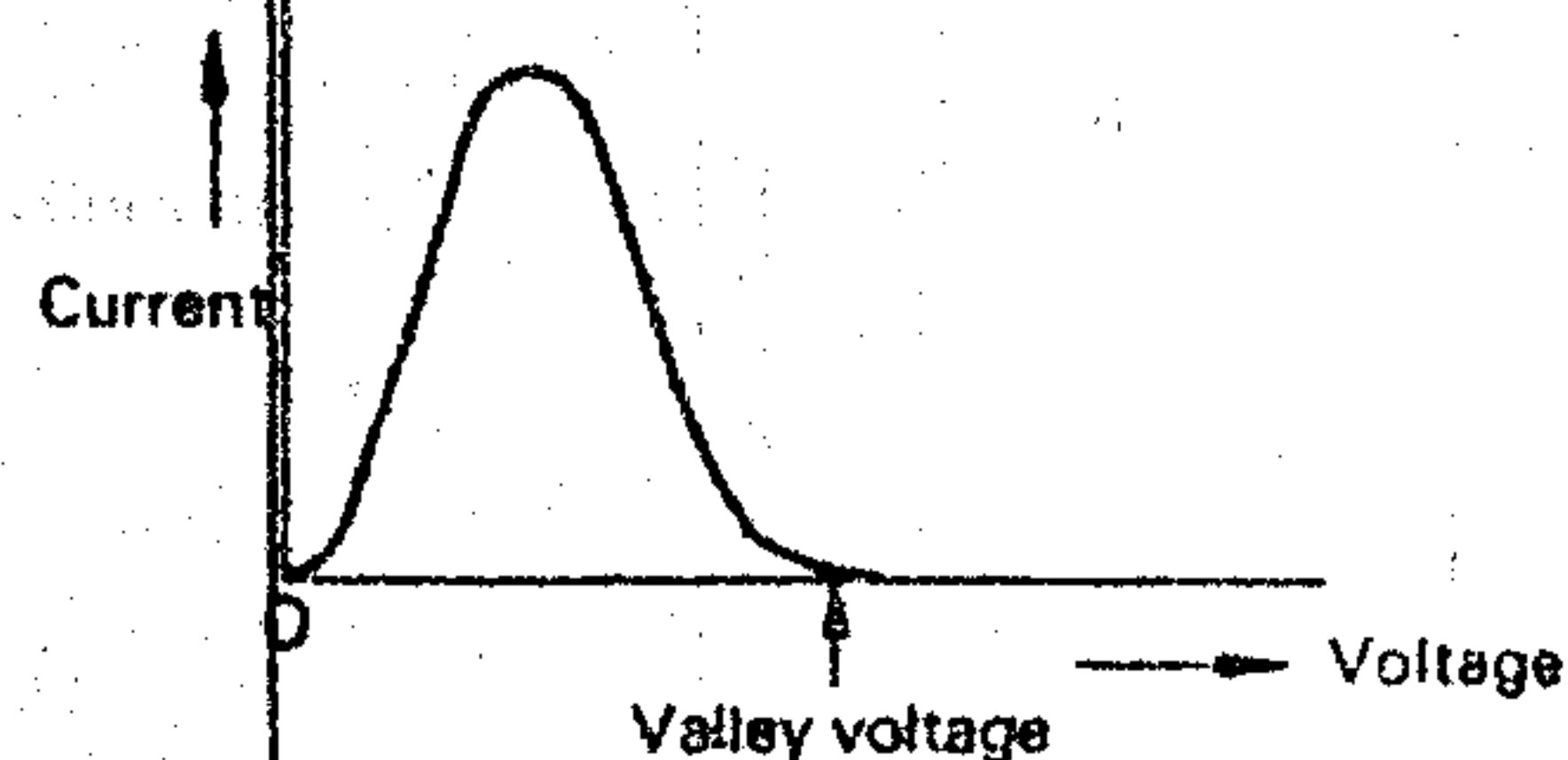
Fig. 11-B Lambda diode characteristics
