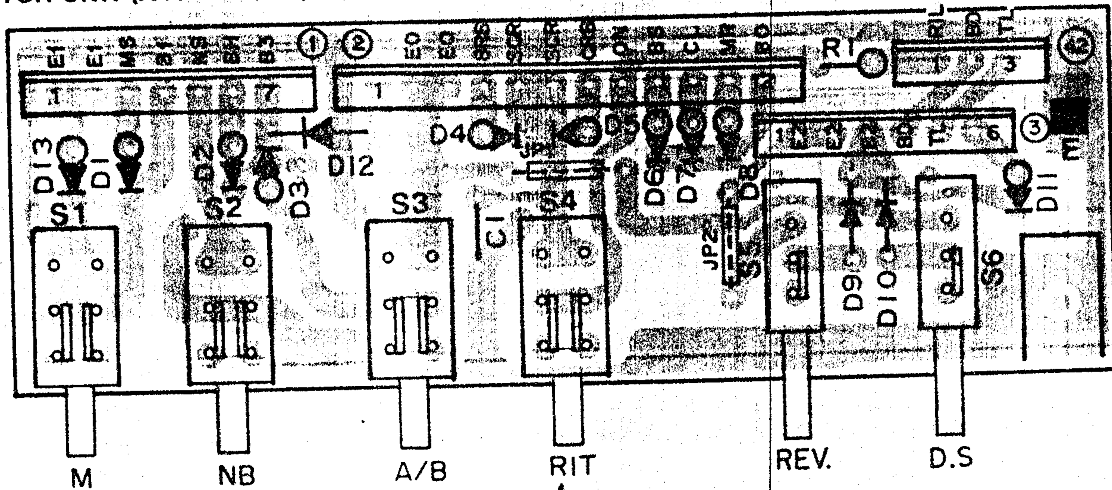
SWITCH UNIT (X41-1400-11) [Component Side View]
