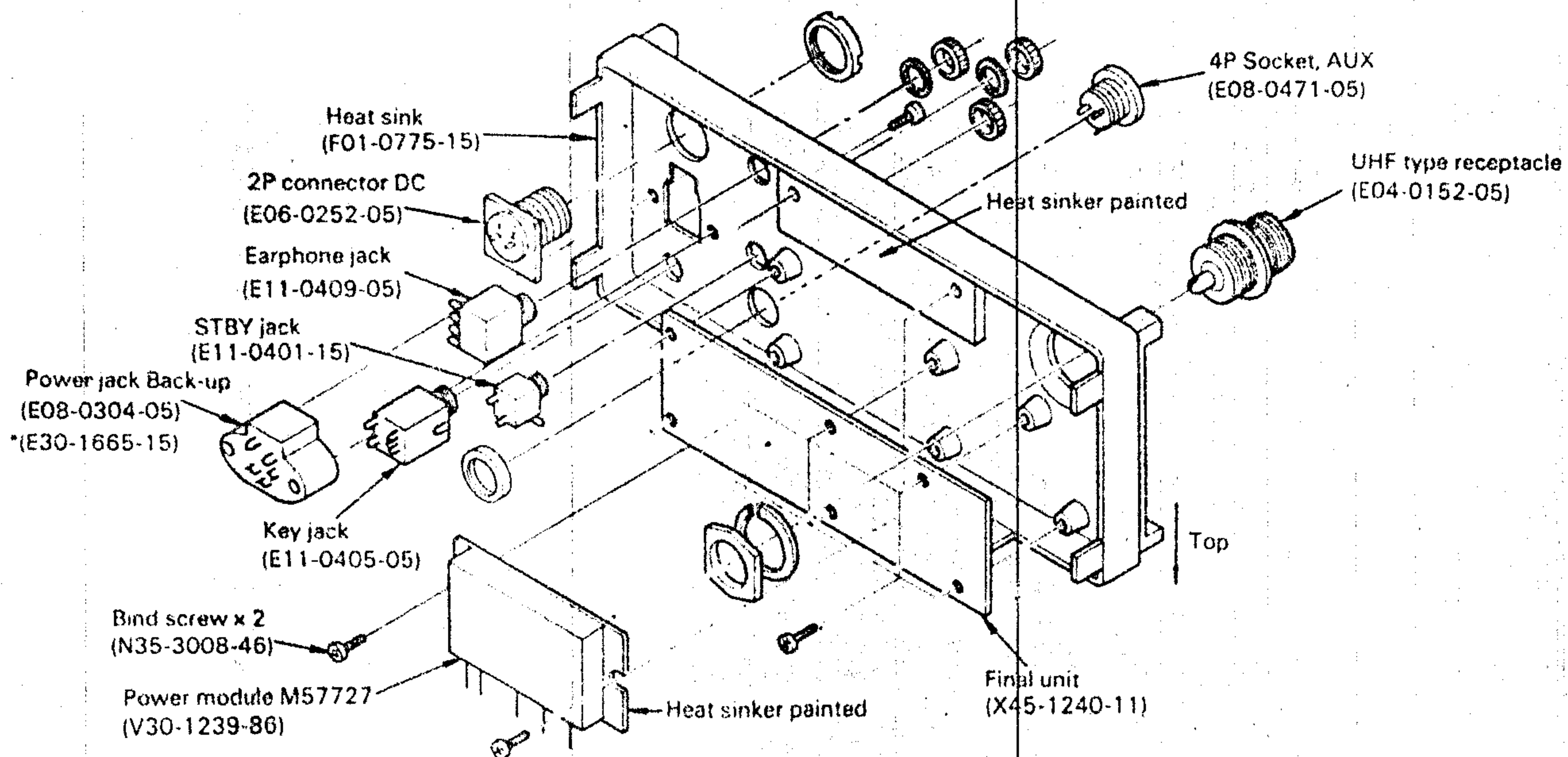
Fig. 22 Rear panel
