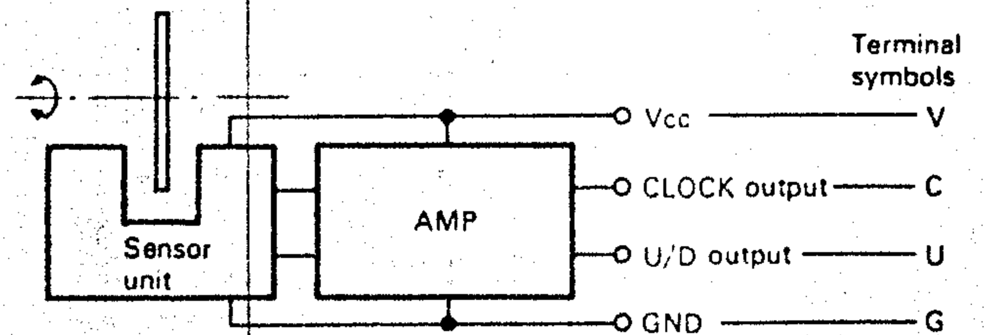
Fig. 13 Rotary encoder (W02-0308-05)
