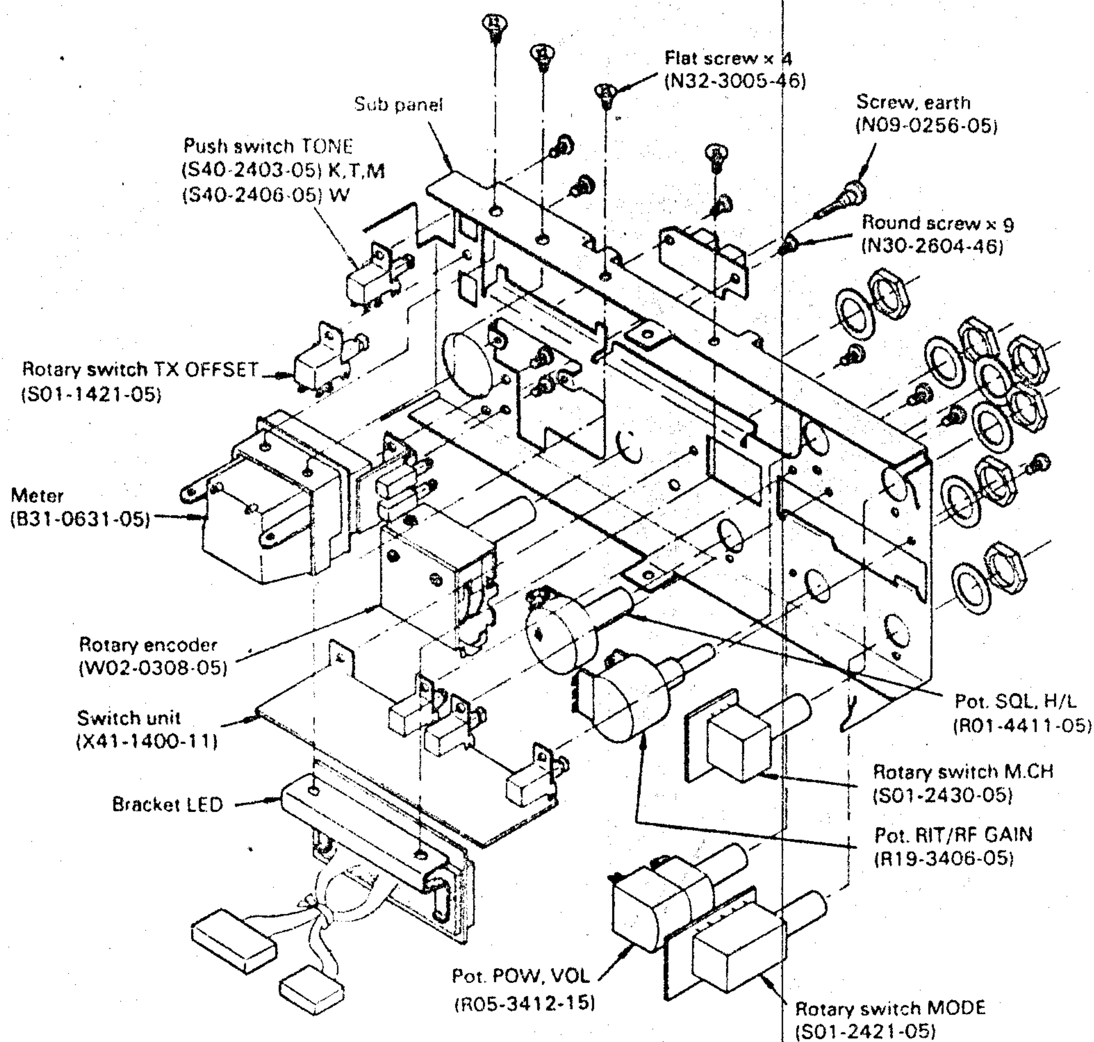
Fig. 21 Sub panel
