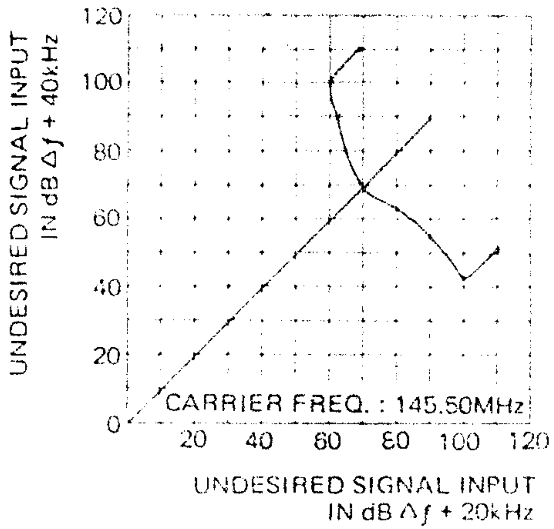
[Inter modulation] FM mode
