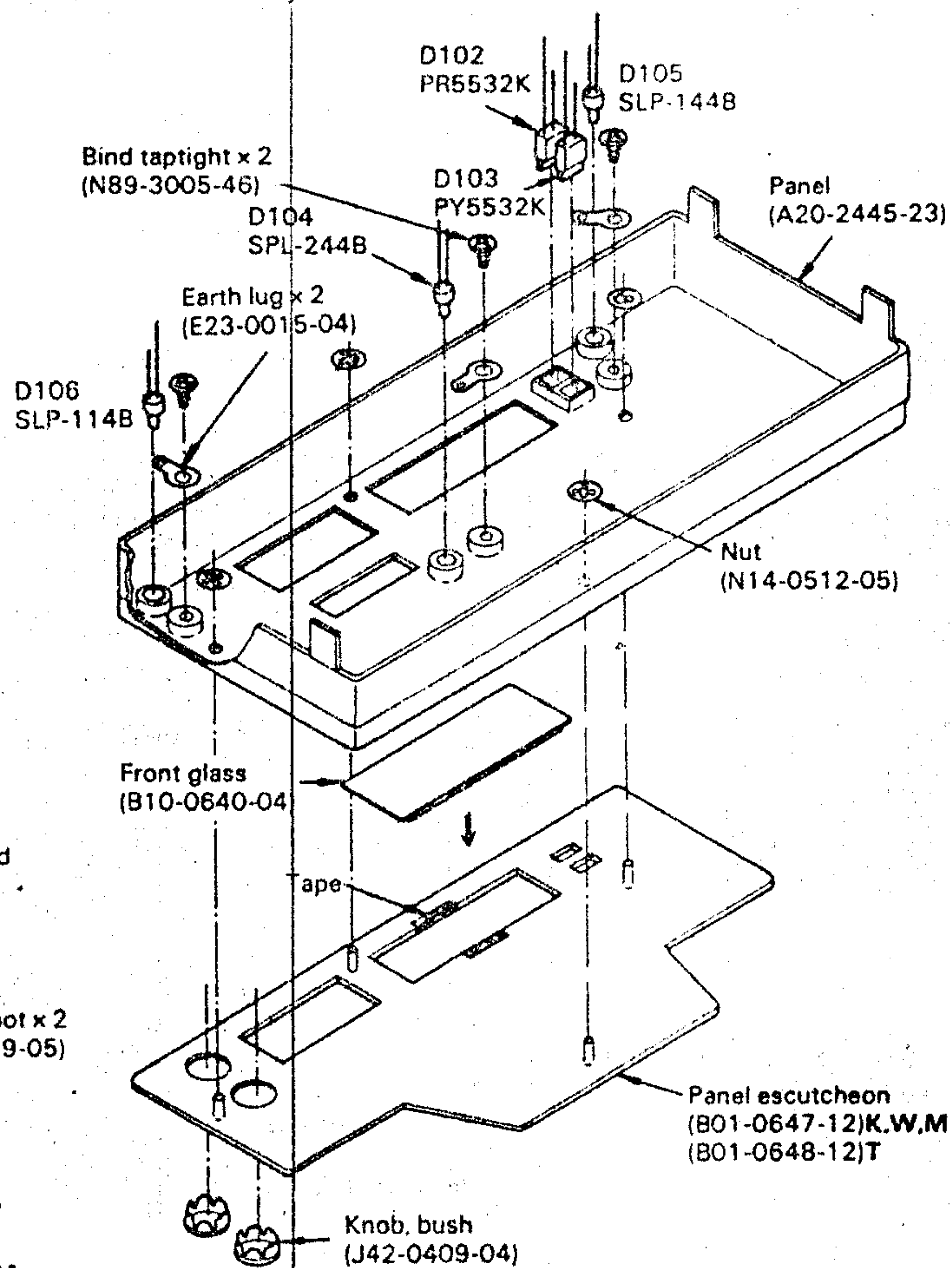
Fig. 19 Panel
