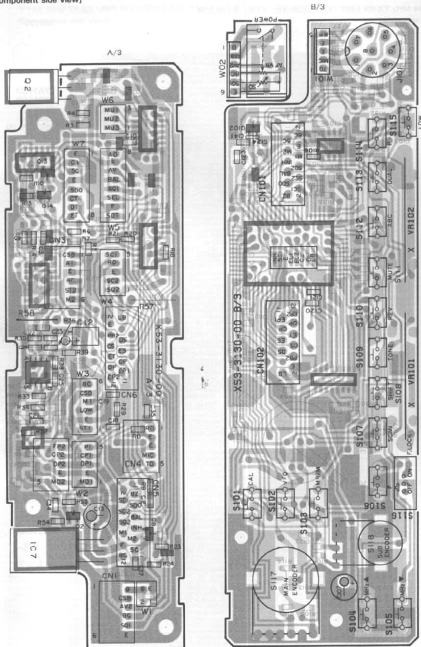
▼CONTROL UNIT (X53-3130-XX) -11:K, -21:M, -51:T, -61:W [Component side view]
